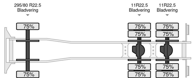
Mercedes-Benz SK 2631 K / 6x4 STEEL SPRINGS
