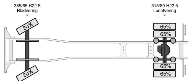
DAF 95.350 - 4x2 - Crane Pesci
