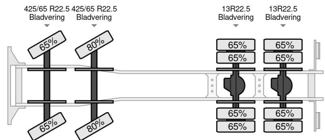
DAF CF85.410 - 8x4 - SOLD SOLD
