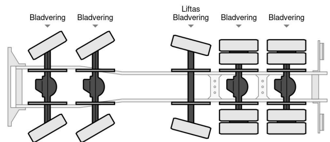
Mercedes-Benz Actros 5044 AK - 10x8 - RESERVED RESER...
