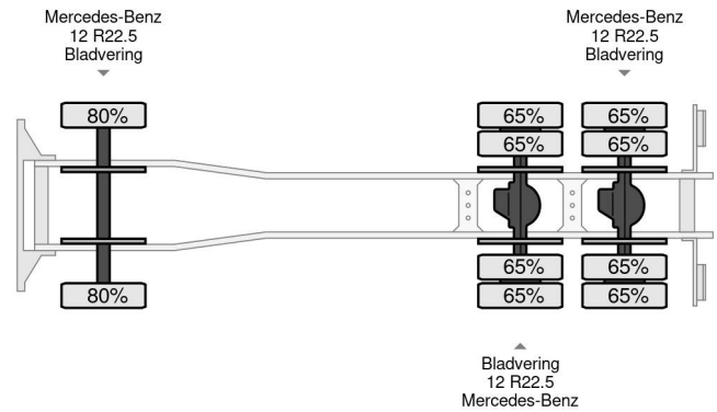
Mercedes-Benz 2628 - 6x4 - Chassis
