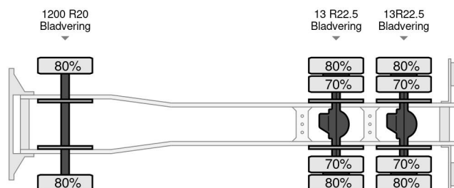
Mercedes-Benz 2628 K - V8 - 6x4 - STEEL SPRINGS
