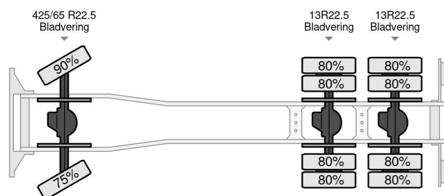
Mercedes-Benz AK 6x6 Steel Springs CRANE TIRRE 131
