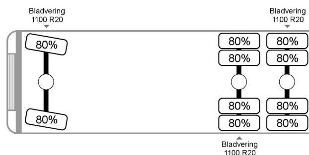
Tatra 815 P 13 - 6x6
