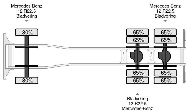
Mercedes-Benz 2628 - 6x4 - Chassis
