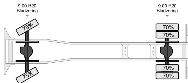
MAN 11.136 Fuel tanker - 4x4
