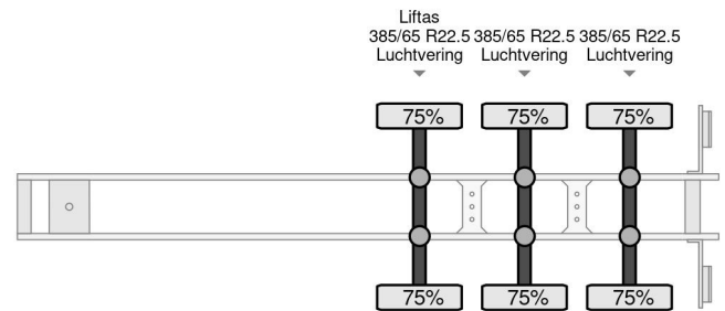
SPITZER EUROVRAC - SK2765CAL - 65M3
