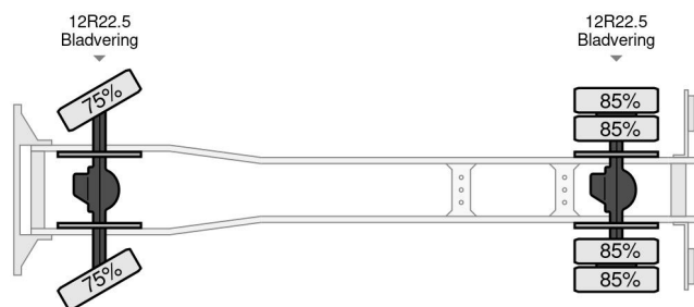
Mercedes-Benz 1824 AK - 4x4 - Fuel tanker
